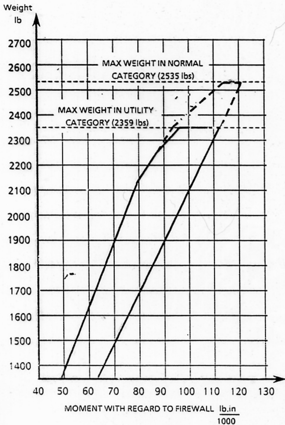
Figure 6.5 - LIMITS WEIGHT / MOMENT
